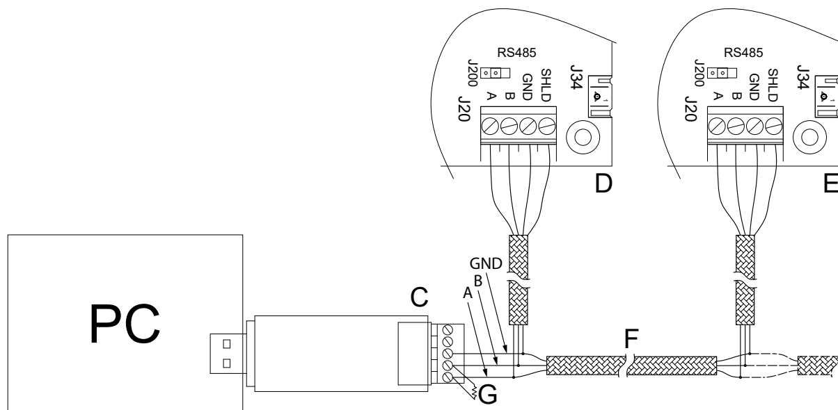
Figure 6.1 Modbus network connection diagram
