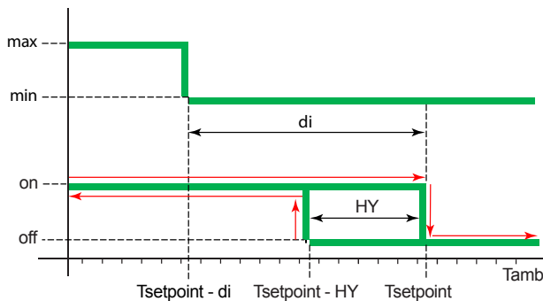
Figure 10.5 Remote independent/assisted mode operation diagram (on/off or modulating)
